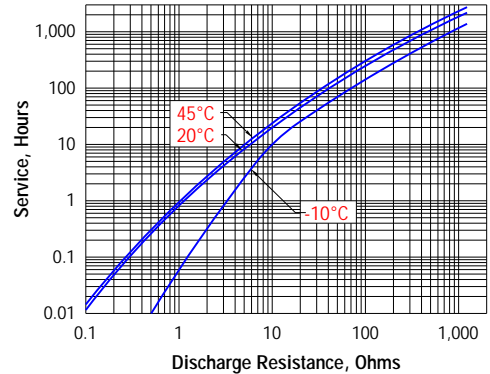
TEMPERATURE EFFECTS Typical Service to 0.8 volts
